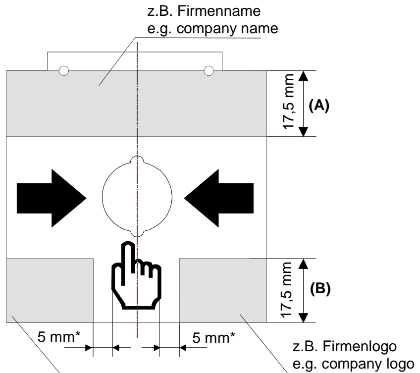
Fig. 1: Labelling of the operation panel from a Manual Call Point (example)
